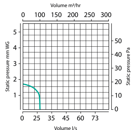
Fan Curves - Performance Graph Low Profile Units
